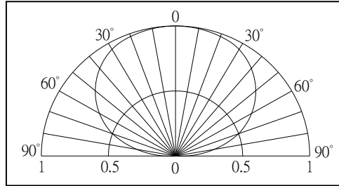
Relative Luminous Intensity
